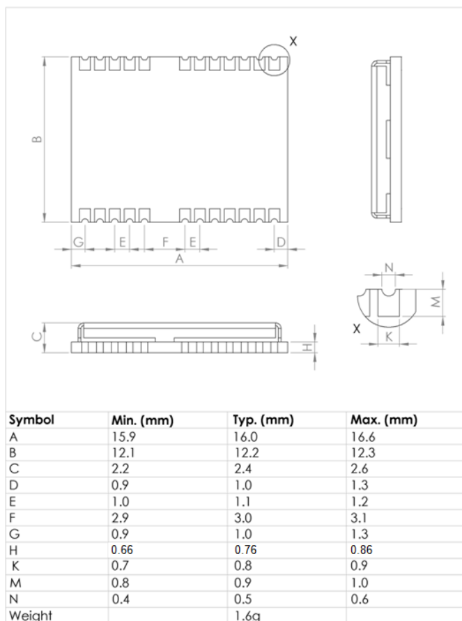
Figure 23: NEO-D9S mechanical dimensions
