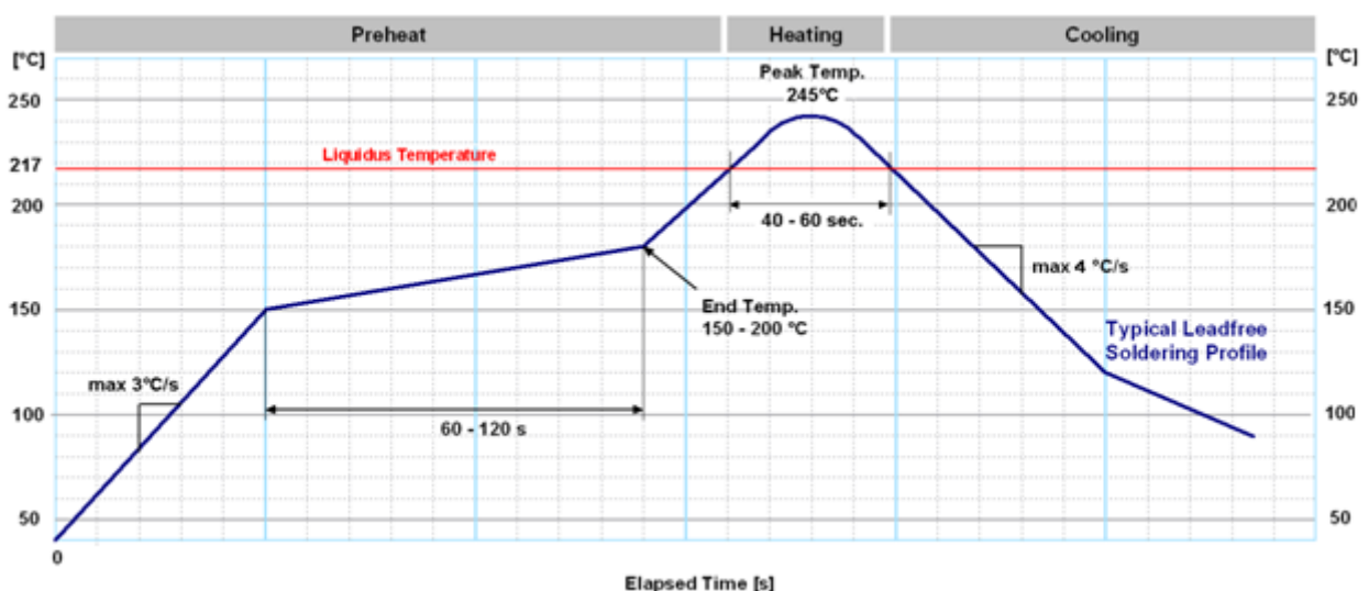
Figure 30: Soldering profile
